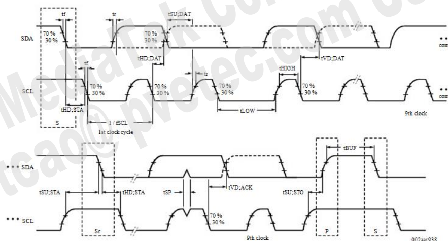
Figure 4-7. I2C AC timing diagram of F/S mode
