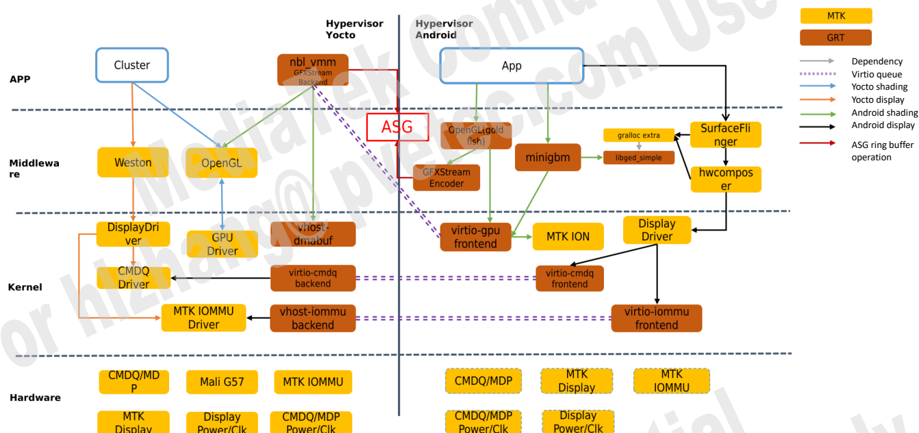
Figure 1-1. Hypervisor graphics system framework
