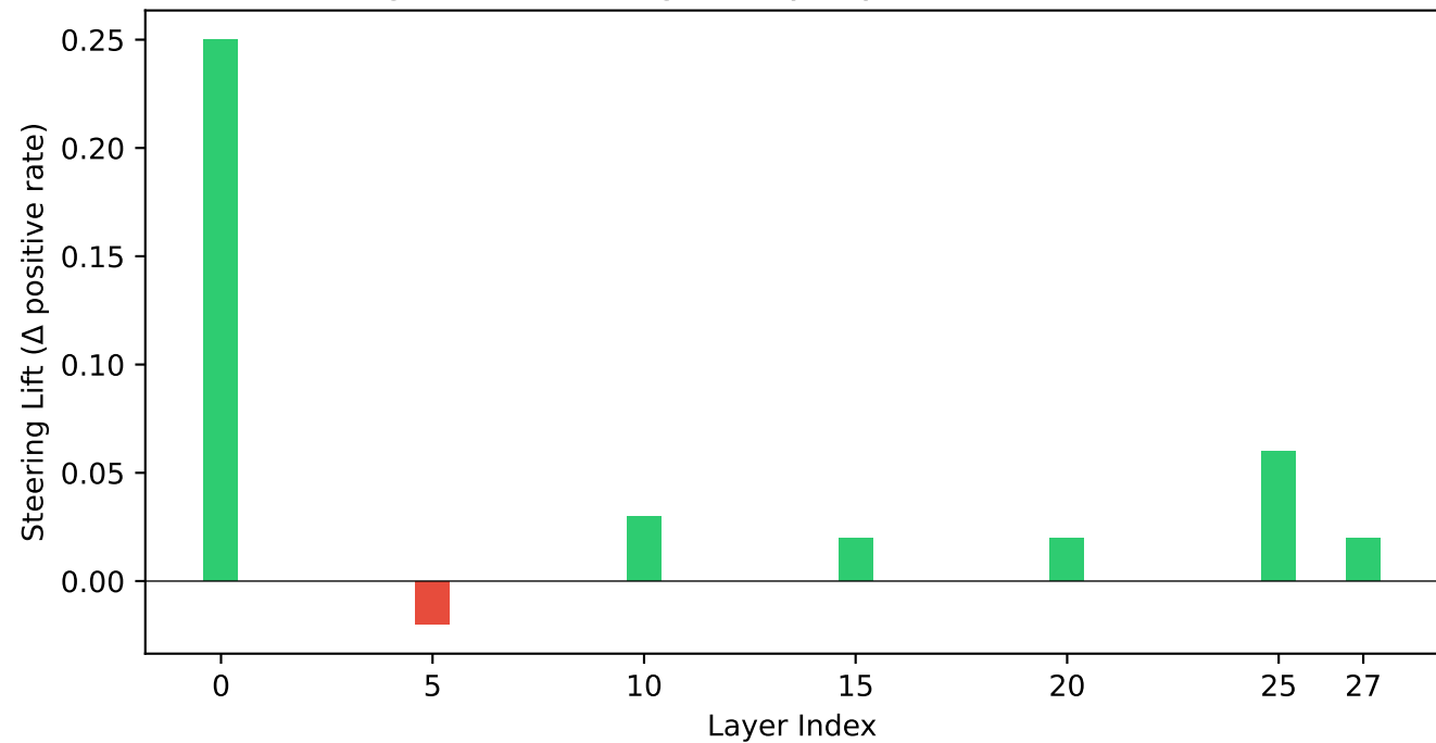
Brightness Steering: Lift by Layer (mean-diff, \epsilon=0.5 )
