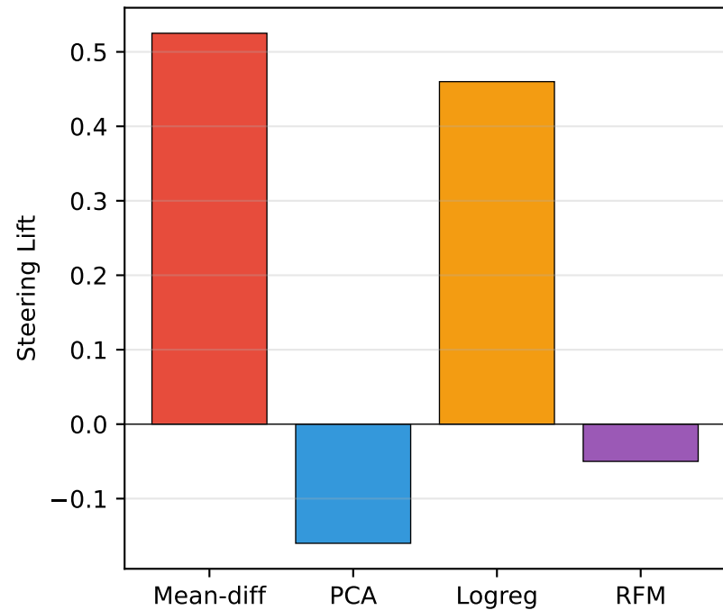
(c) Steering Effectiveness
