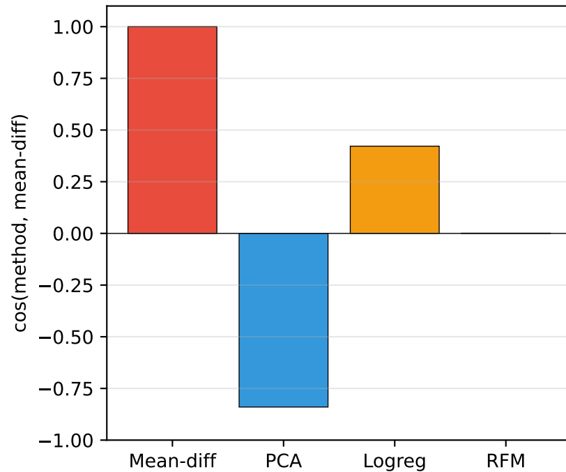
(b) Alignment with Mean-Diff
