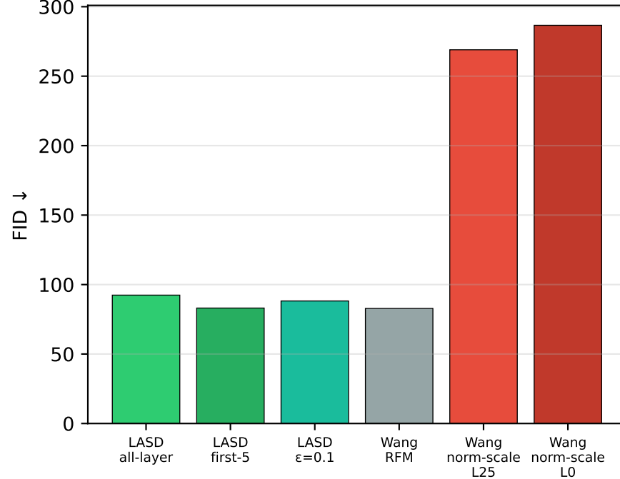
(b) Quality Degradation
