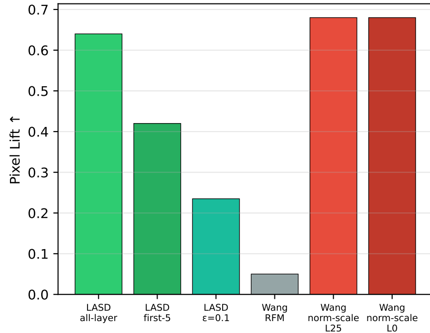
(a) Concept Shift
