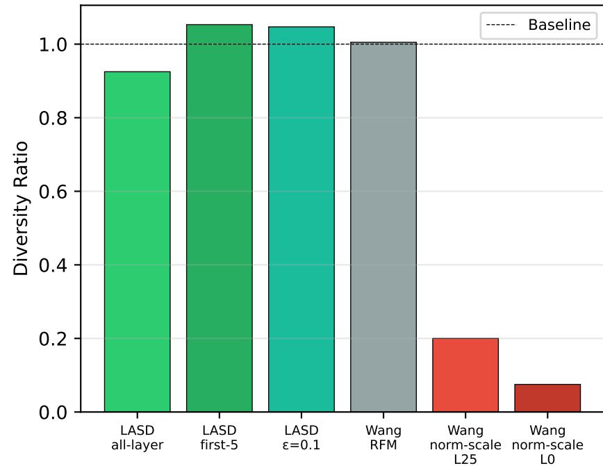
(c) Sample Diversity
