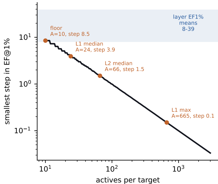
One extra hit moves EF@1% by this much
