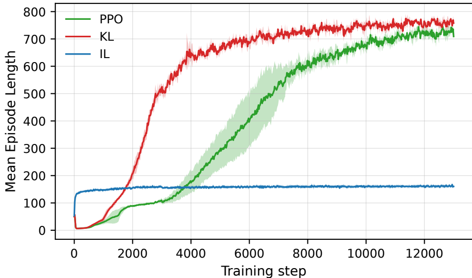
Teacher-Student Ablation: Mean Episode Length
