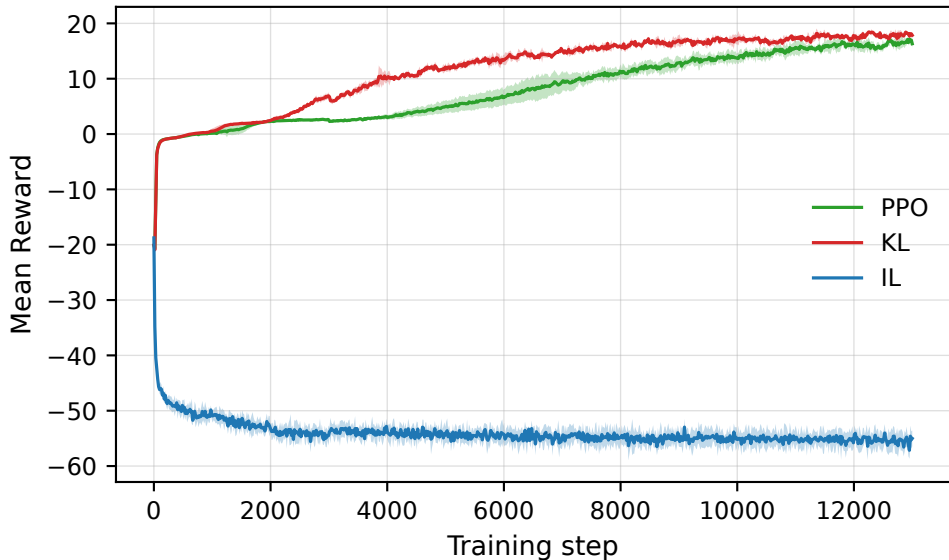
Teacher-Student Ablation: Mean Reward
