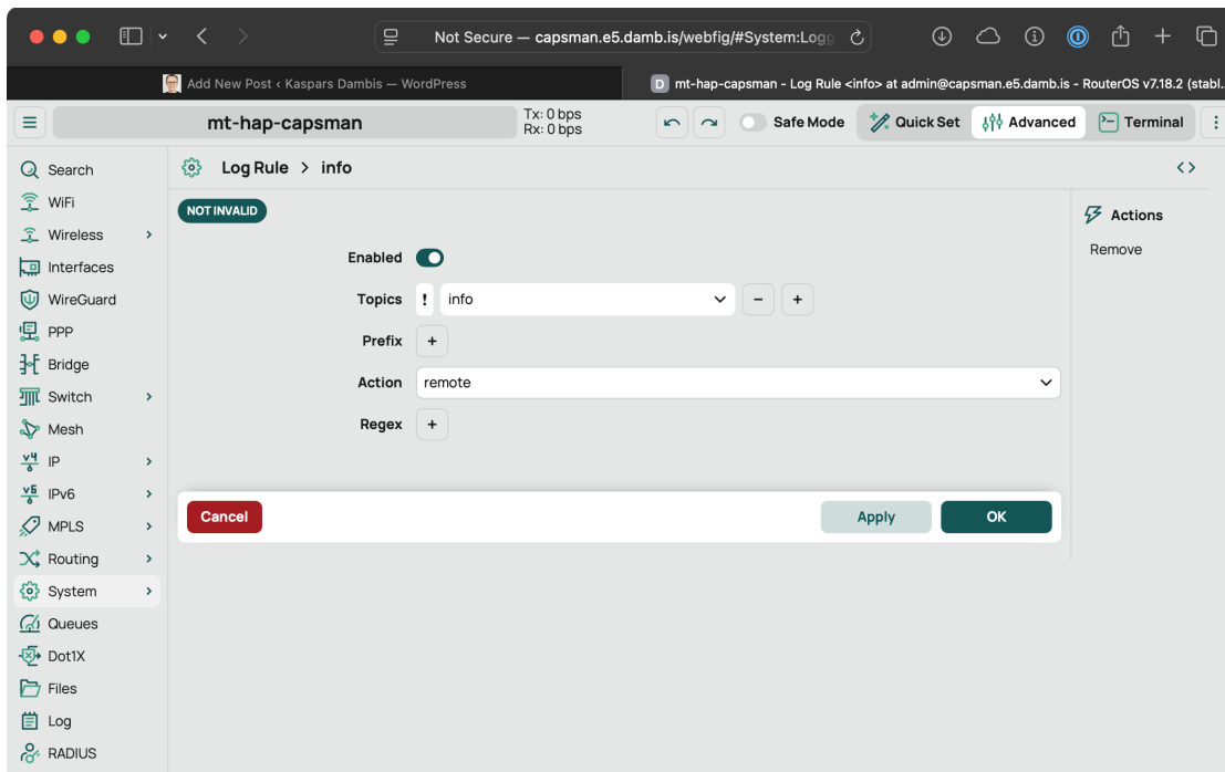
Figure 2: System > Logging > Rules — one rule per topic (here topics=info, action=remote).
