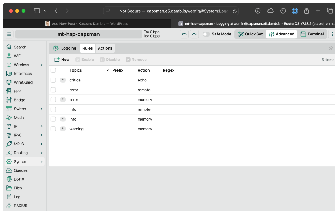
Figure 3: System > Logging > Rules — separate row per topic (RouterOS ANDs topics on one row). Every row for a topic you want forwarded must point at your remote action.
