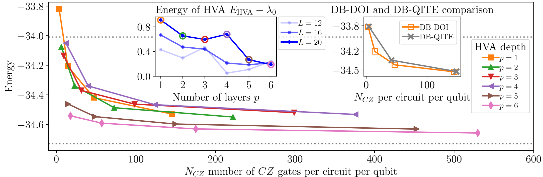
DB-DOI for L = 20 qubit \hat{H}_{\text{XXX}} with HVA warm-start
