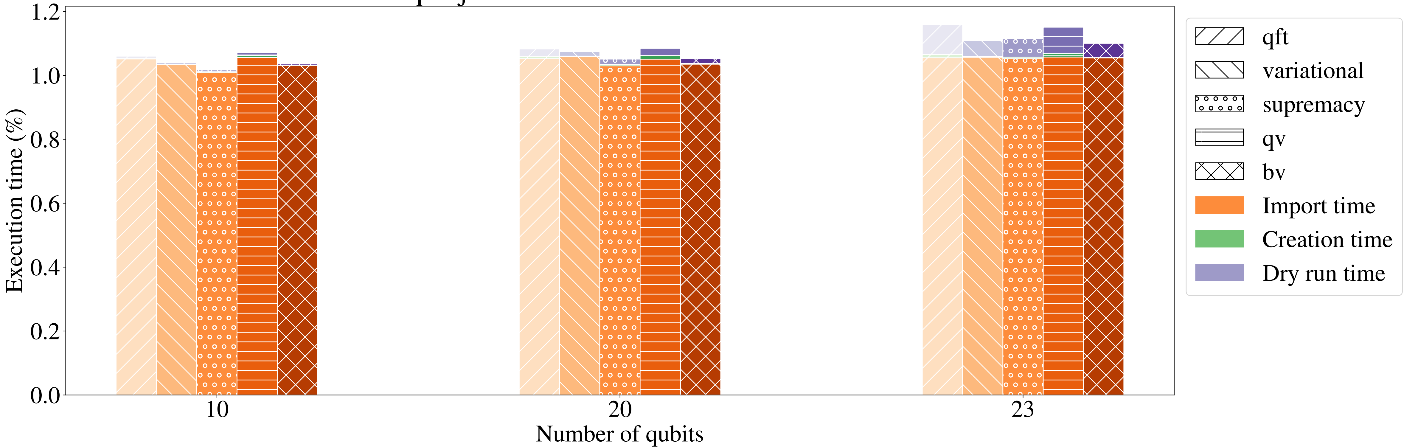
qibojit - Breakdown of total run time
