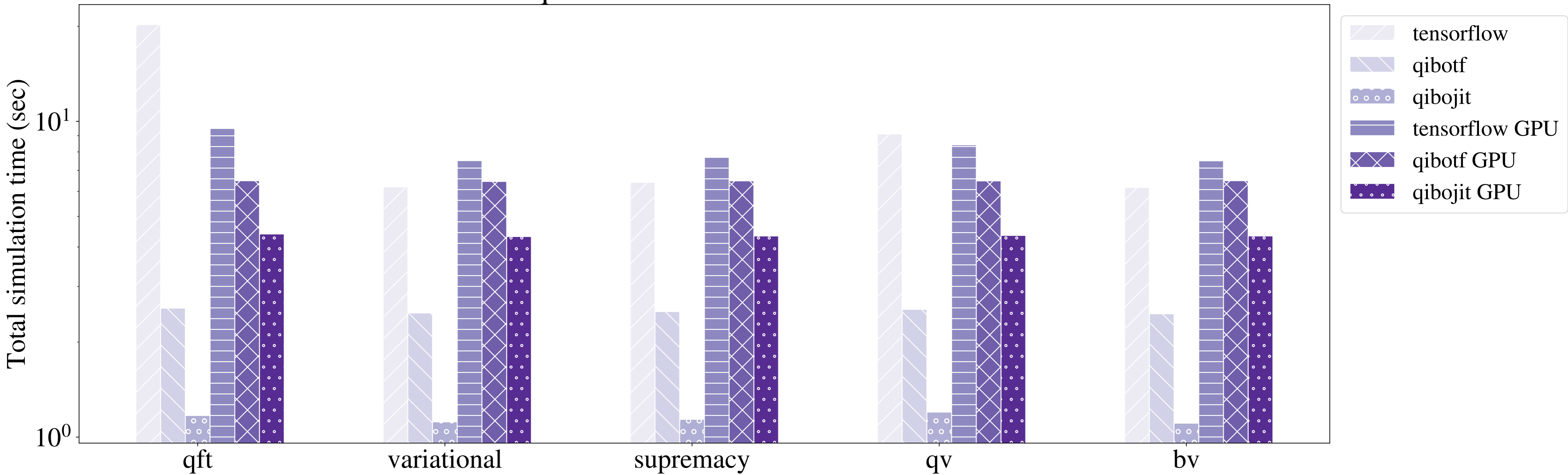
23 qubits - Total simulation time
