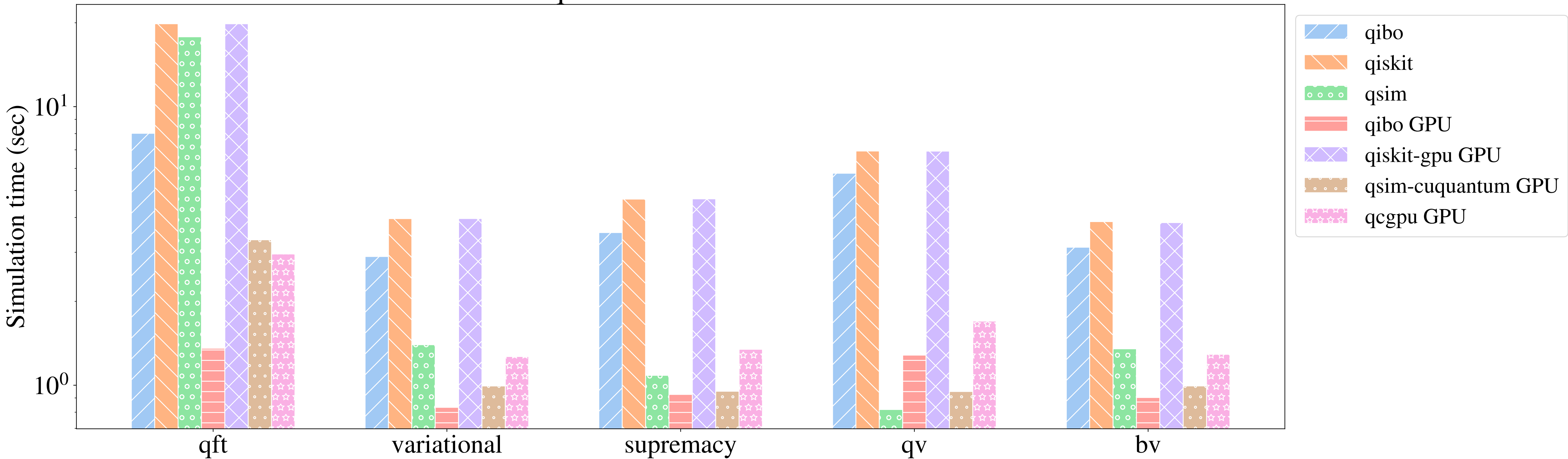
28 qubits - Simulation time
