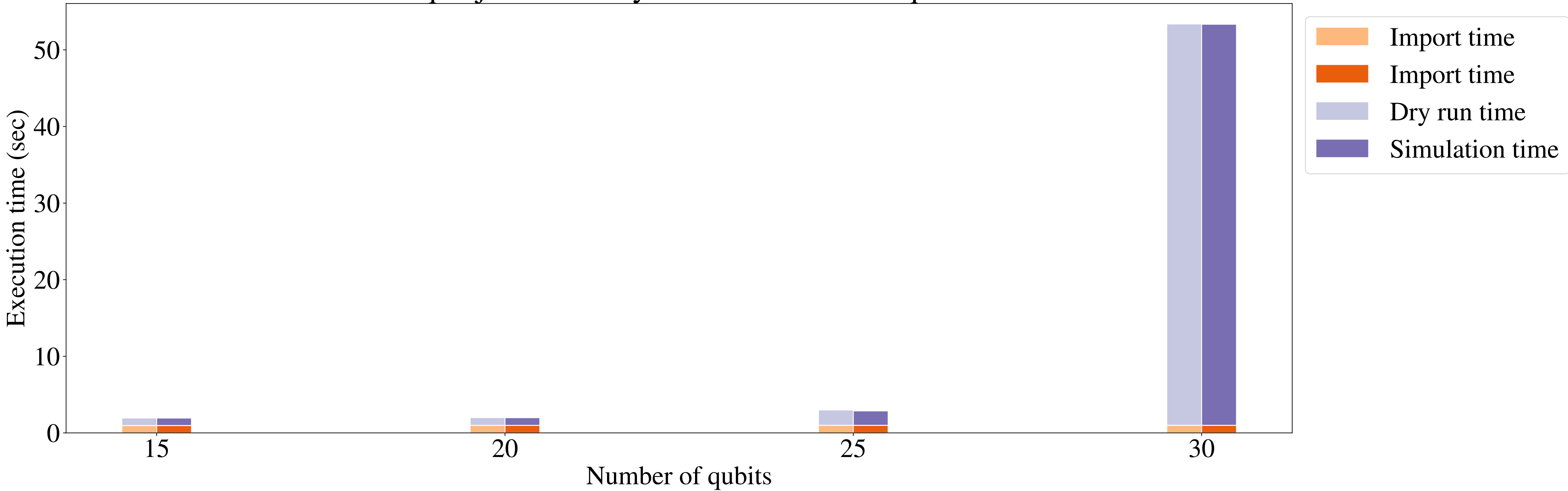
qibojit CPU - Dry run vs simulation - qft
