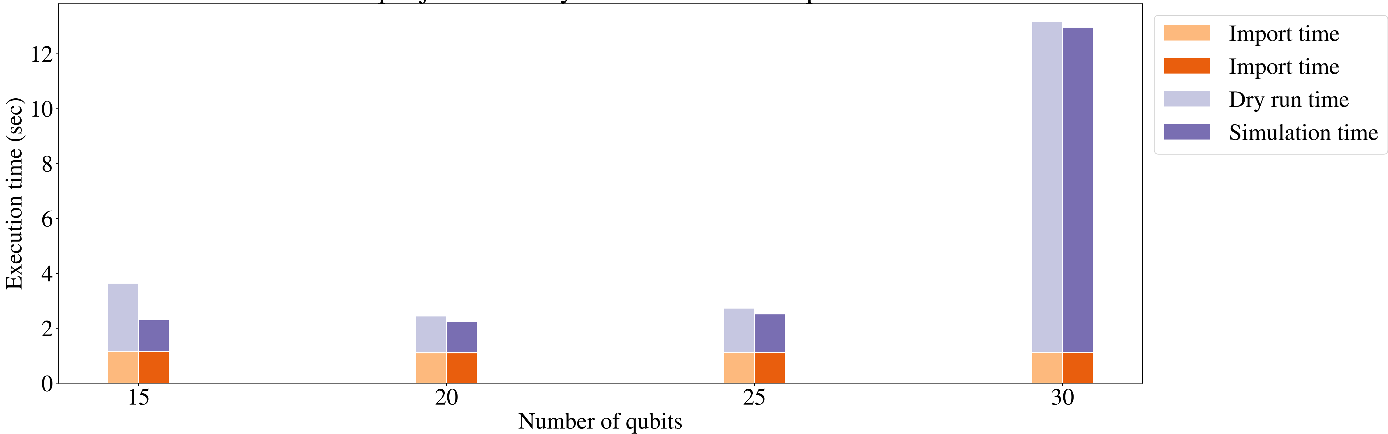
qibojit GPU - Dry run vs simulation - qft
