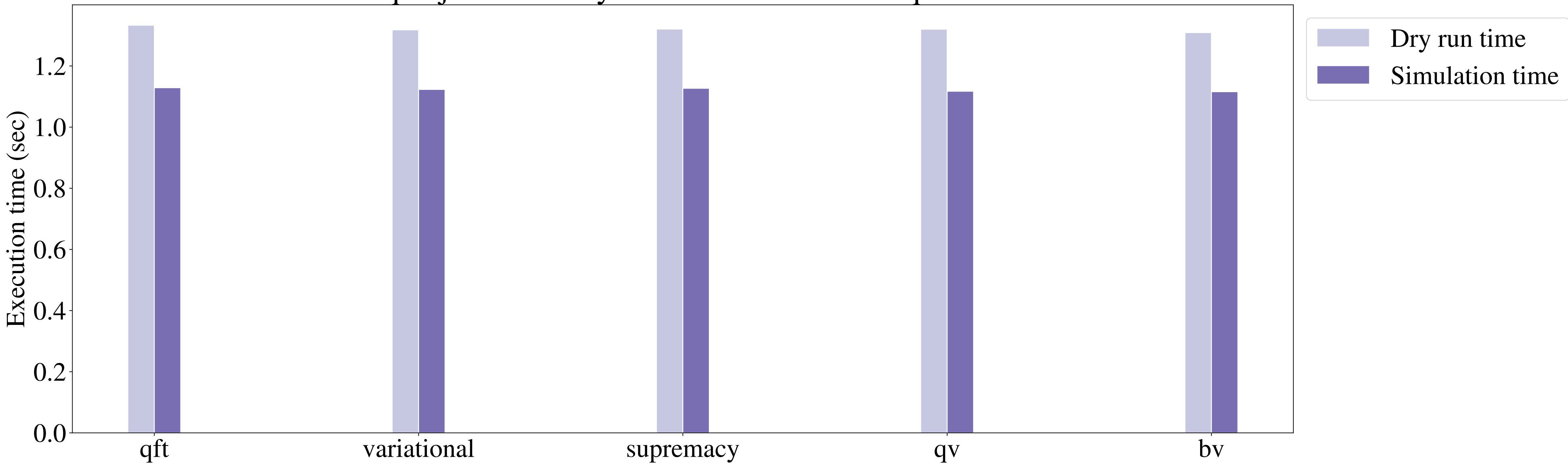
qibojit GPU - Dry run vs simulation - 20 qubits
