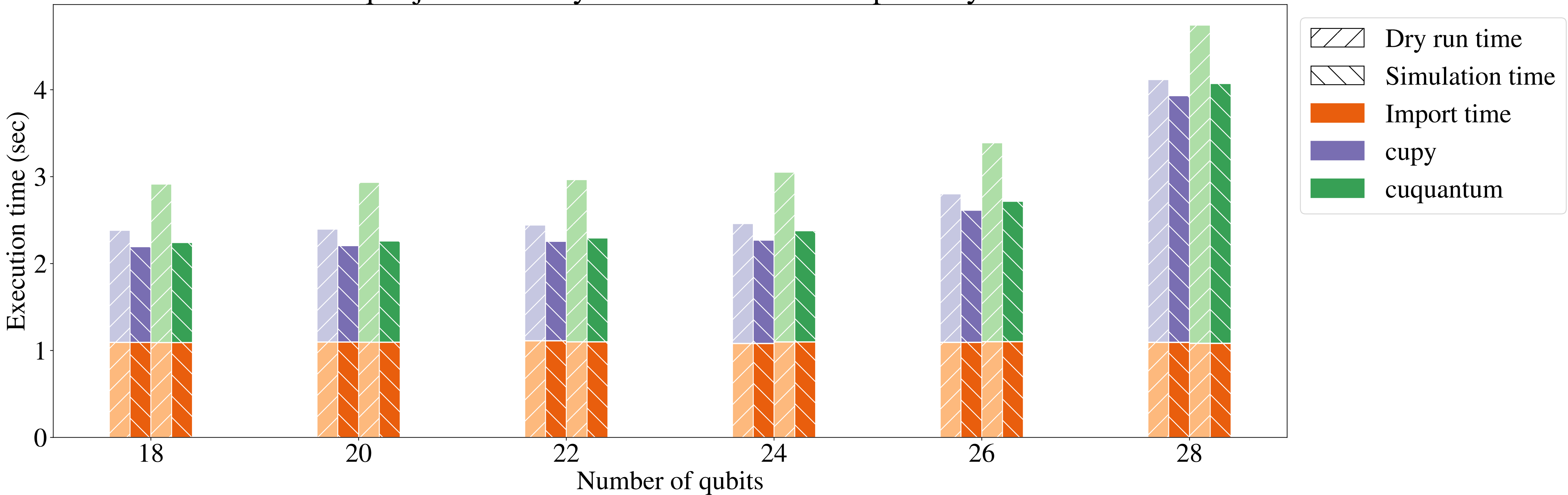
qibojit GPU - Dry run vs simulation - supremacy
