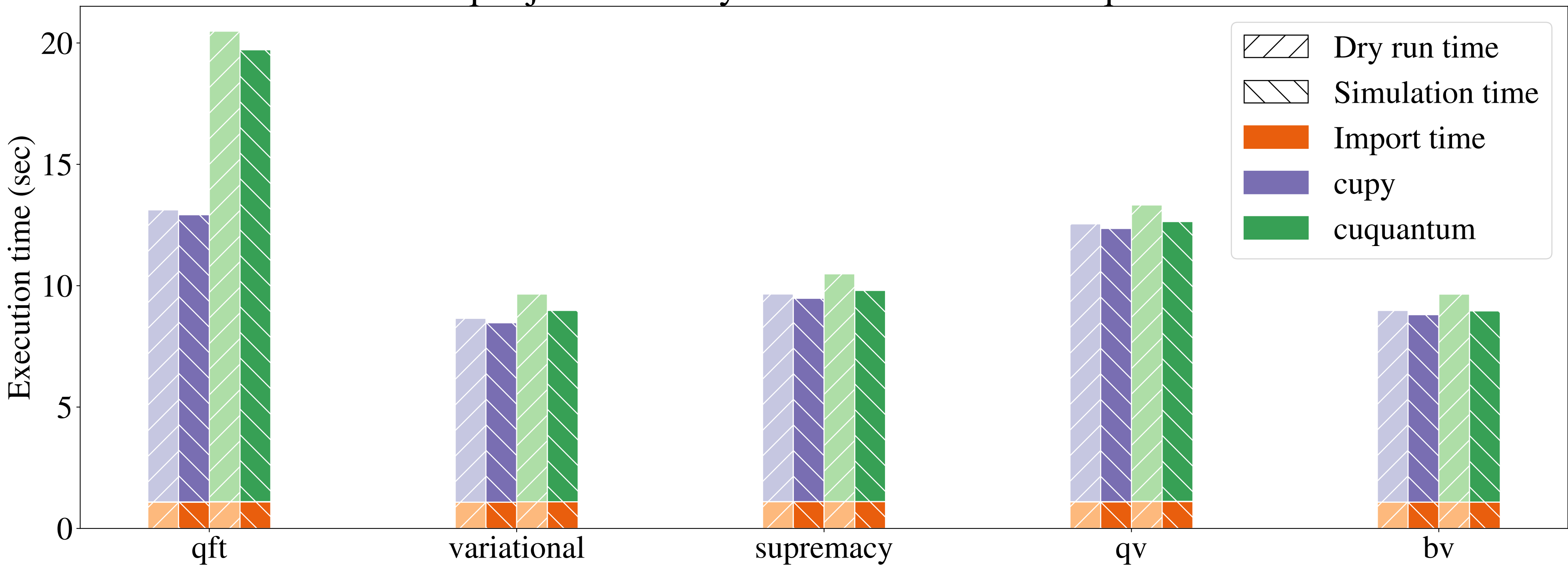
qibojit GPU - Dry run vs simulation - 30 qubits
