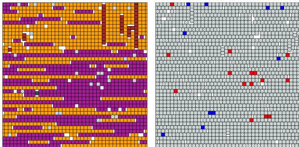
2 \times 2 \times 2 cubes on \mathbb{Z}^3 , high-density columnar phase
