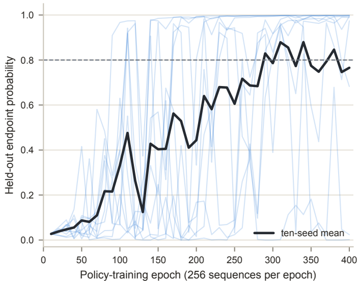
a Locked replication trajectories
