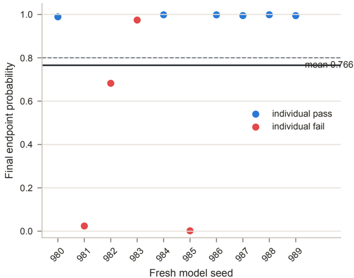
b Six of ten seeds pass the individual rule
