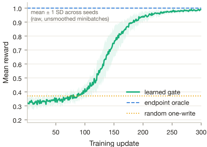
(a) Optimization discovers the high-reward regime
