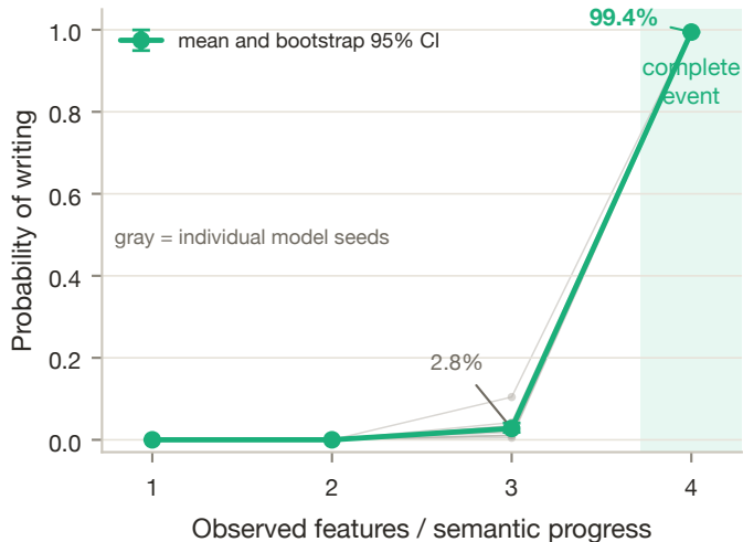
(b) The learned gate writes at completion
