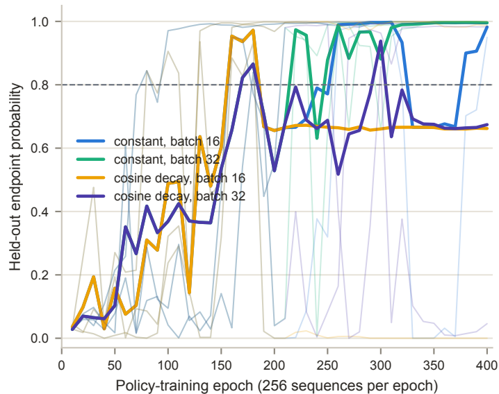
a Full-mixture learning trajectories
