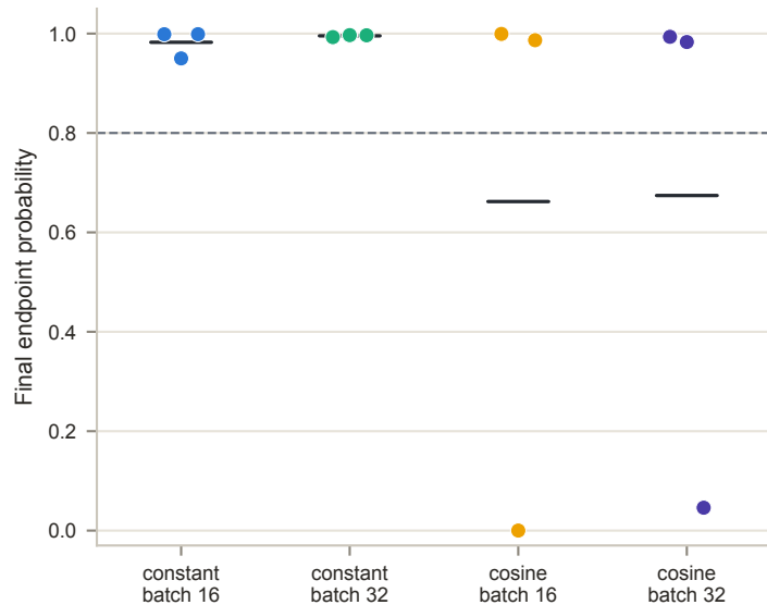
b Final checkpoints for all paired seeds
