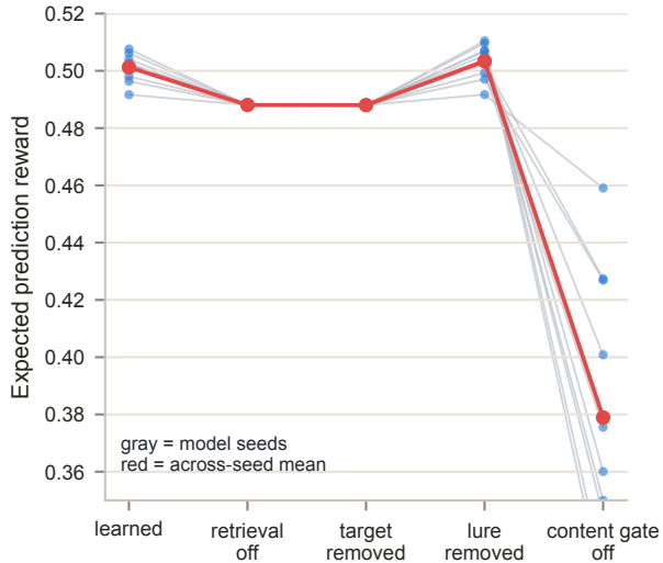
b Paired DM causal ablations
