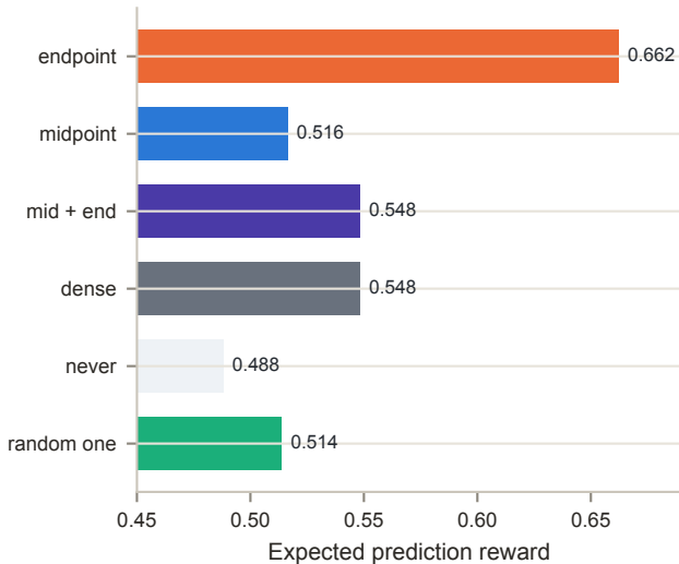
a Forced schedules: endpoint is best in DM
