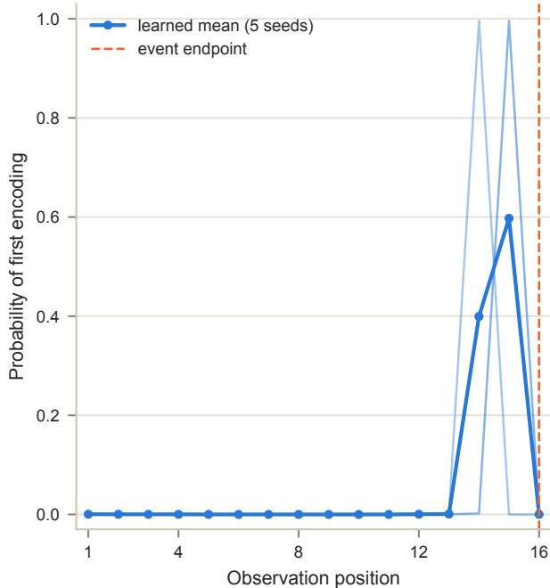
a Exact mixed reward has a better endpoint solution but gradients stop one or two steps early
