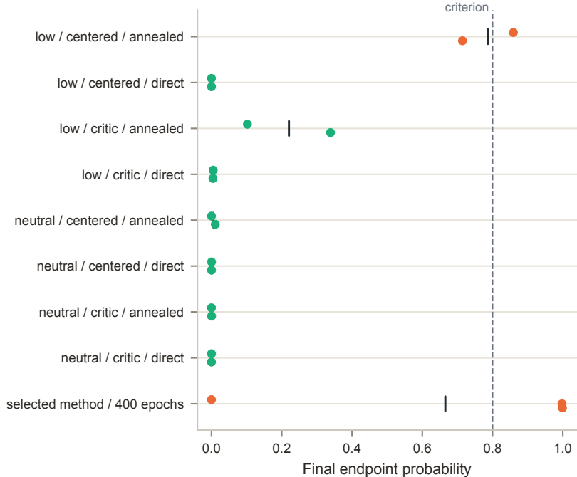
b A bounded credit screen finds a promising but unstable full-mixture method
