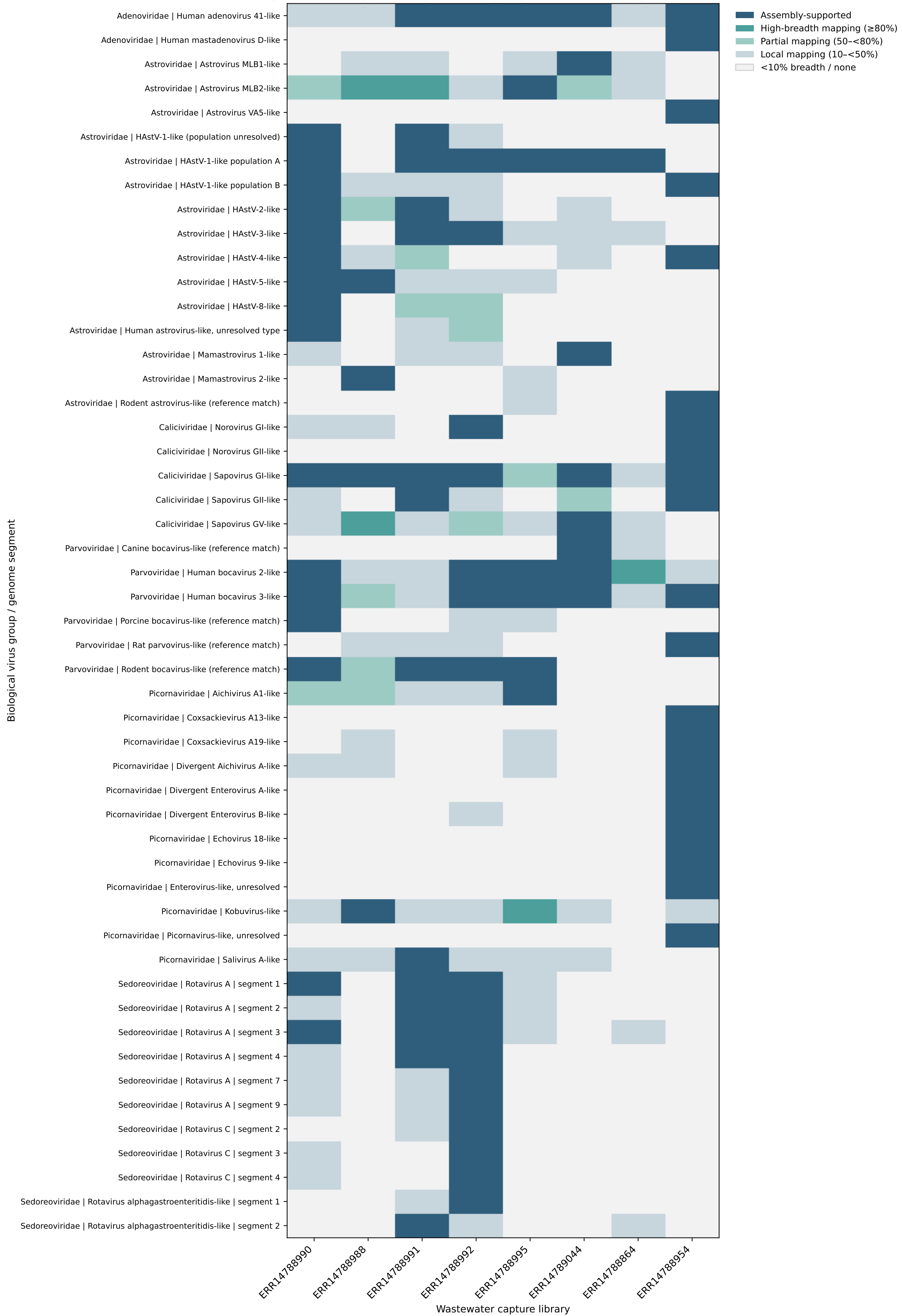
Integrated assembly and competitive-mapping evidence across eight capture libraries
