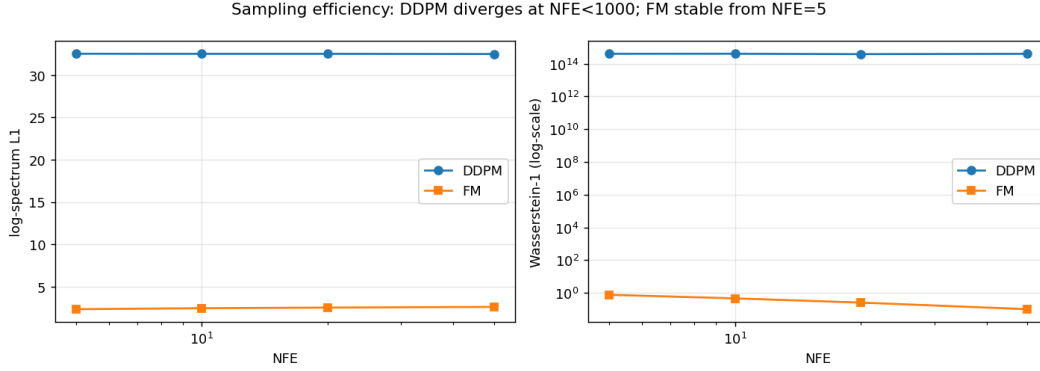
Figure 5: Sampling efficiency vs. NFE. Flow Matching is stable from NFE= 5 and monotonically improves; DDIM from the DDPM checkpoint diverges for every NFE < 1000 tested (Wasserstein-1 \sim 10^{14} , plotted on a log scale).
