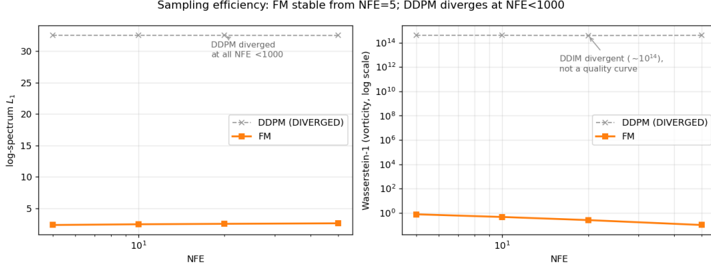
Figure 5: Sampling efficiency vs. NFE. Flow Matching (orange) is stable from NFE= 5 (Wasserstein-1 = 0.77) and monotonically improves to 0.10 at NFE= 50. DDIM sampling from the DDPM checkpoint diverges at every sub-1000 NFE tested (Wasserstein-1 \sim 10^{14} ), so the gray dashed line is plotted as a divergence indicator rather than as a performance curve. The contrast should be read as “FM remains usable where DDPM is not,” not as a trade-off curve for DDPM.
