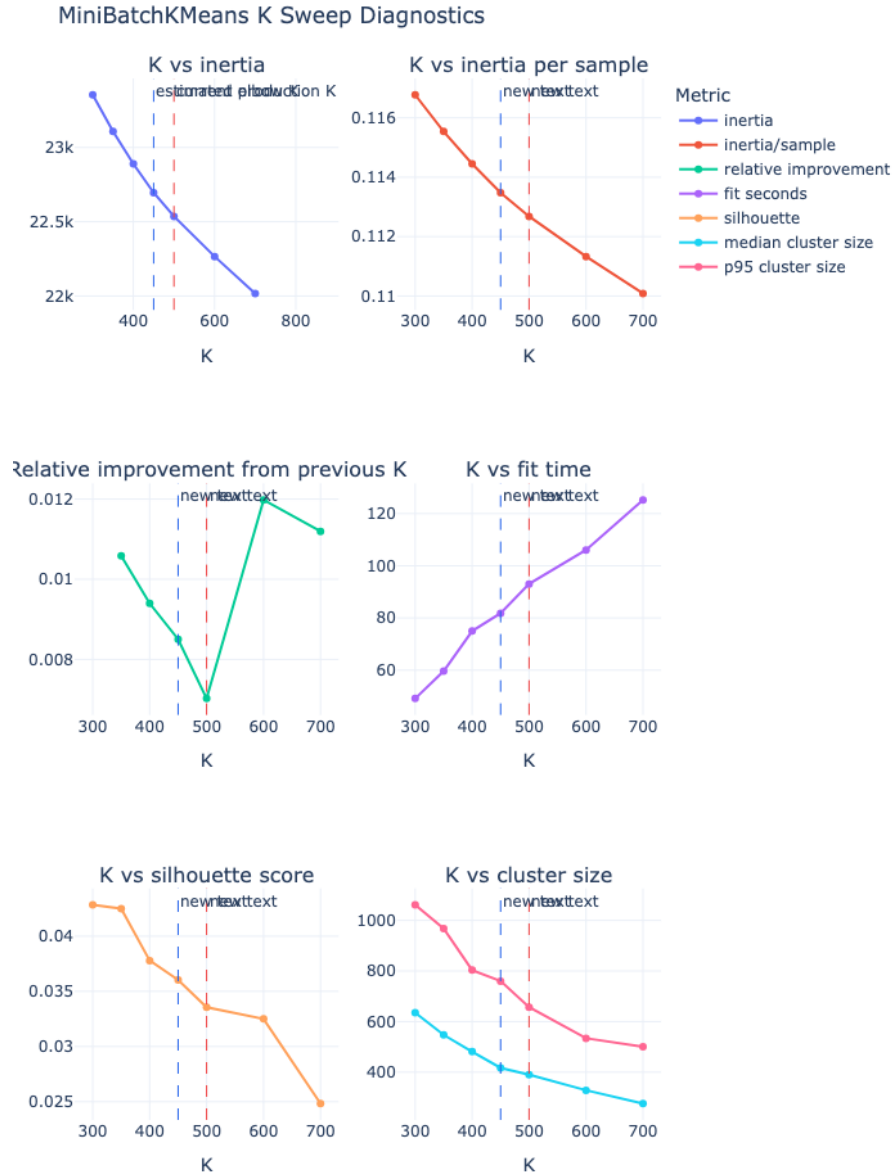
Figure 1: MiniBatchKMeans diagnostic sweep. The elbow region is around K_c = 450 – 500 ; the production spatial index uses K_c = 500 .
