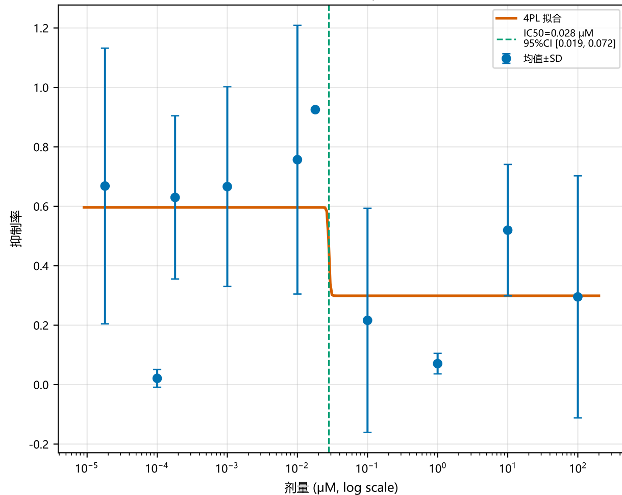
剂量-响应曲线 (4PL, HillSlope=43.30, n=34)
