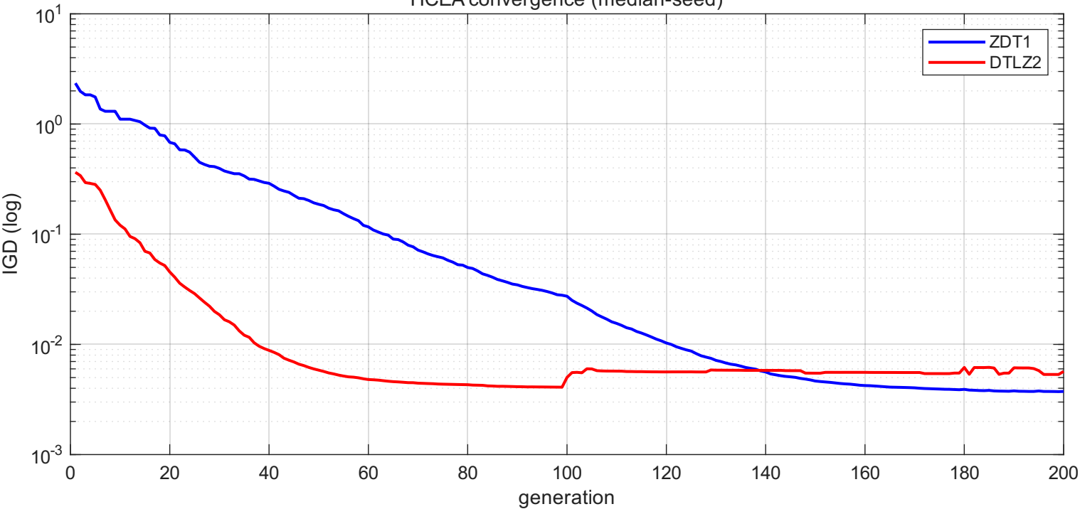
HCEA convergence (median-seed)
