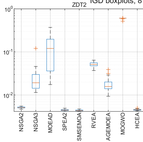
IGD boxplots, 8 problems (log scale)
