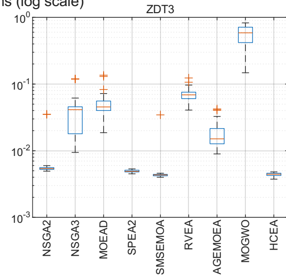
IGD boxplots, 8 problems (log scale)
