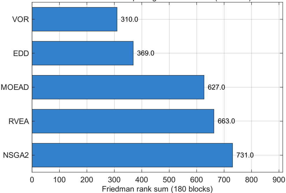
Friedman rank test: per-algorithm rank sum (30 seeds)
