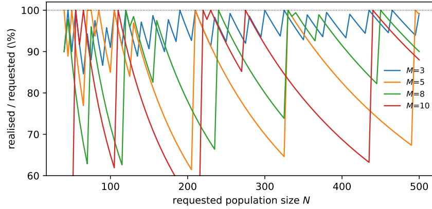
Figure 1 Realised population size as a fraction of the requested size for the default reference-vector constructor of PlatEMO 4.16. The realised count is a step function of the request; at the sizes used in practice it lies below the request, and the deficit grows with the number of objectives
