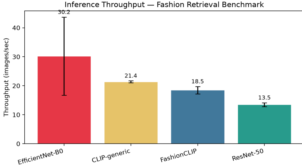
Figure 45: Throughput comparison across four evaluated models. EfficientNet-B0 leads at 30.2 img/s, followed by CLIP-generic (21.4), Fashion-CLIP (18.5), and ResNet-50 (13.5).
