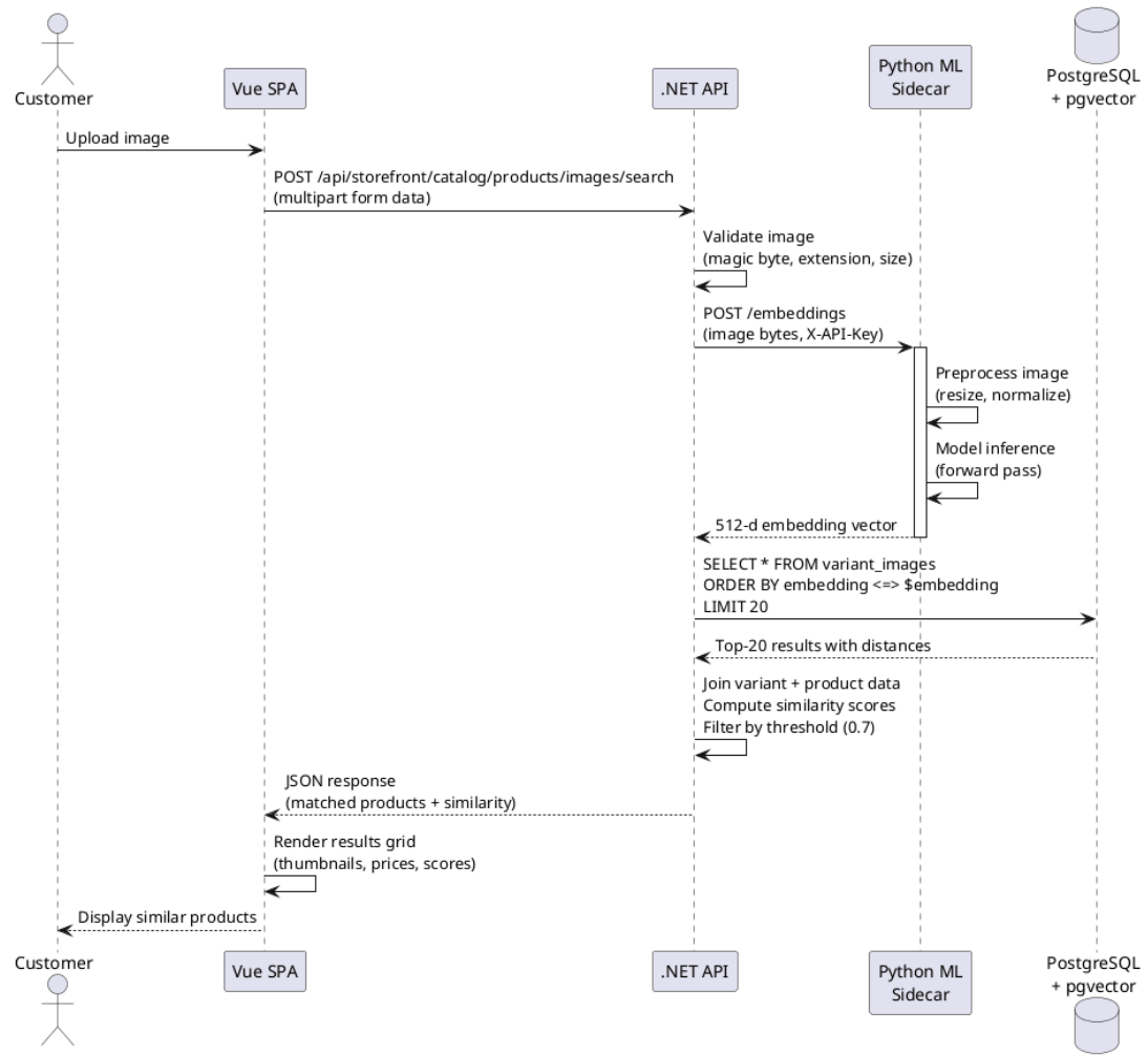
Figure 41: CBIR search sequence: end-to-end flow spanning customer upload, embedding extraction, pgvector search, and ranked results rendering.
