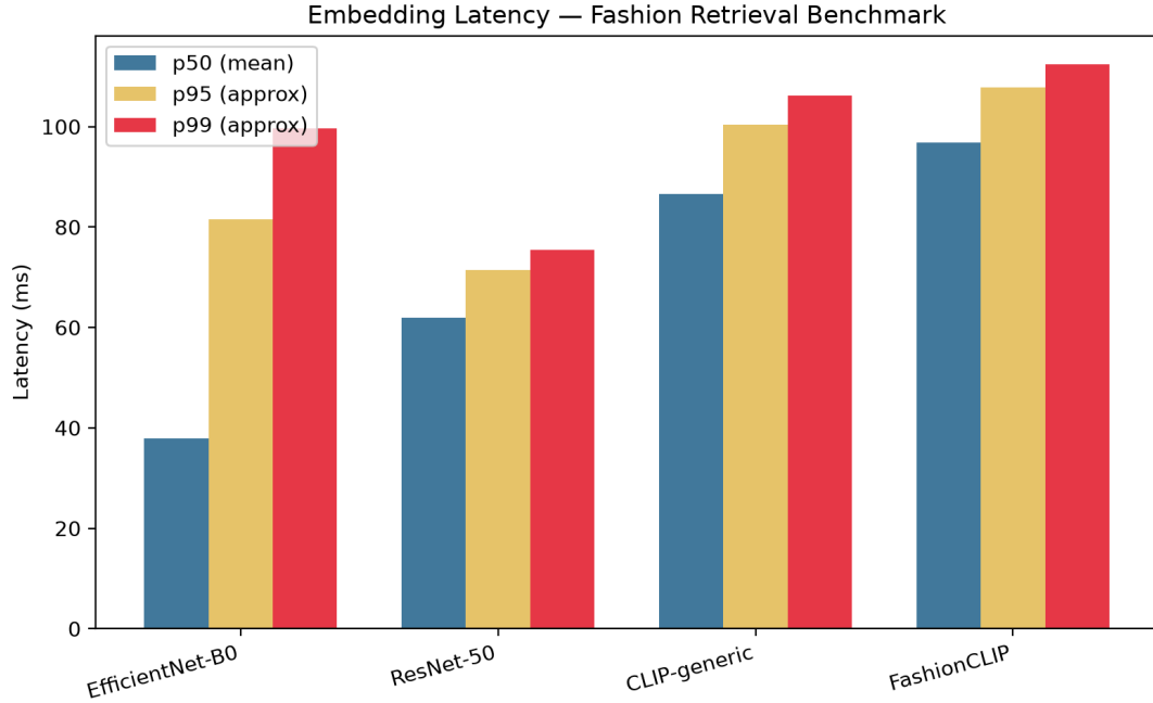
Figure 44: Inference latency comparison across four evaluated models. EfficientNet-B0 leads at 37.8 ms, followed by ResNet-50 (61.9 ms), CLIP-generic (86.6 ms), and Fashion-CLIP (96.8 ms).
