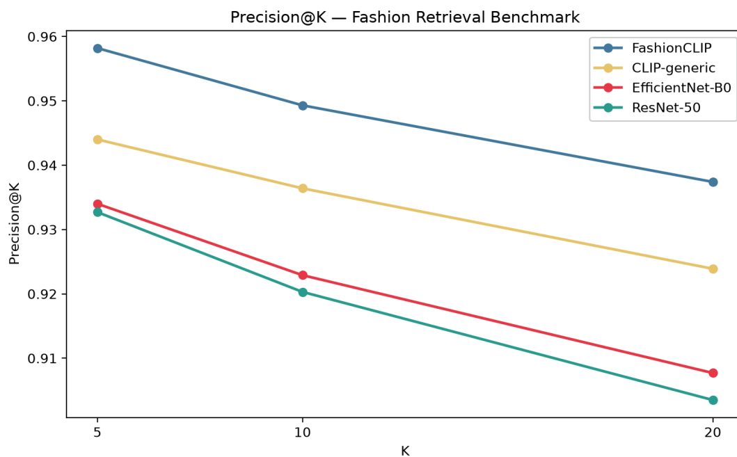
Figure 43: Precision at K (K = 5, 10, 20) across four evaluated models. Fashion-CLIP maintains the highest precision at every retrieval depth.
