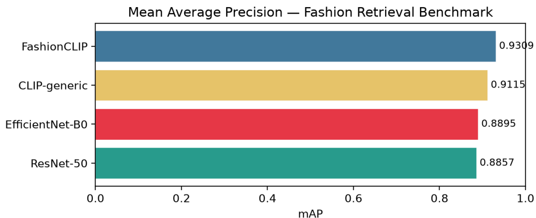
Figure 42: mAP comparison across four evaluated models. Fashion-CLIP leads at 0.9309, followed by CLIP-generic (0.9115), EfficientNet-B0 (0.8895), and ResNet-50 (0.8857).
