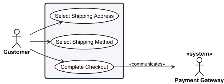
Figure 24: Use case diagram for Checkout Flow (UC-STR-CHK).
