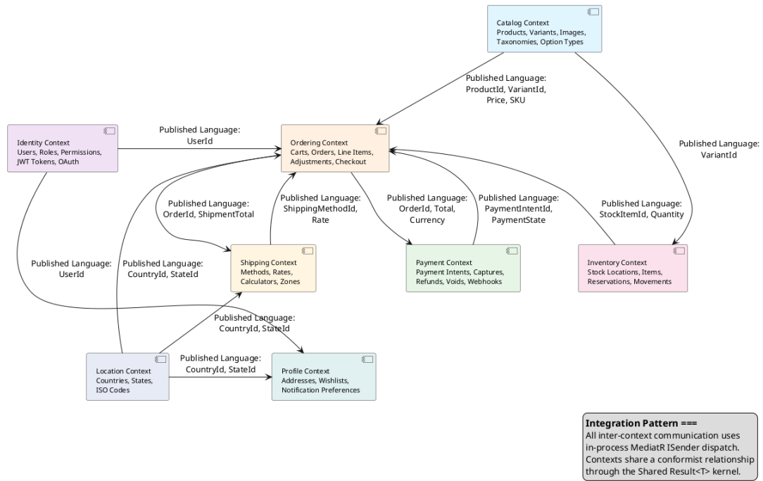
Figure 9: Bounded Context Map showing the eight business contexts and the Published Language identifiers exchanged between them. All integration uses in-process MediatR dispatch; no context directly references another context's namespace.
