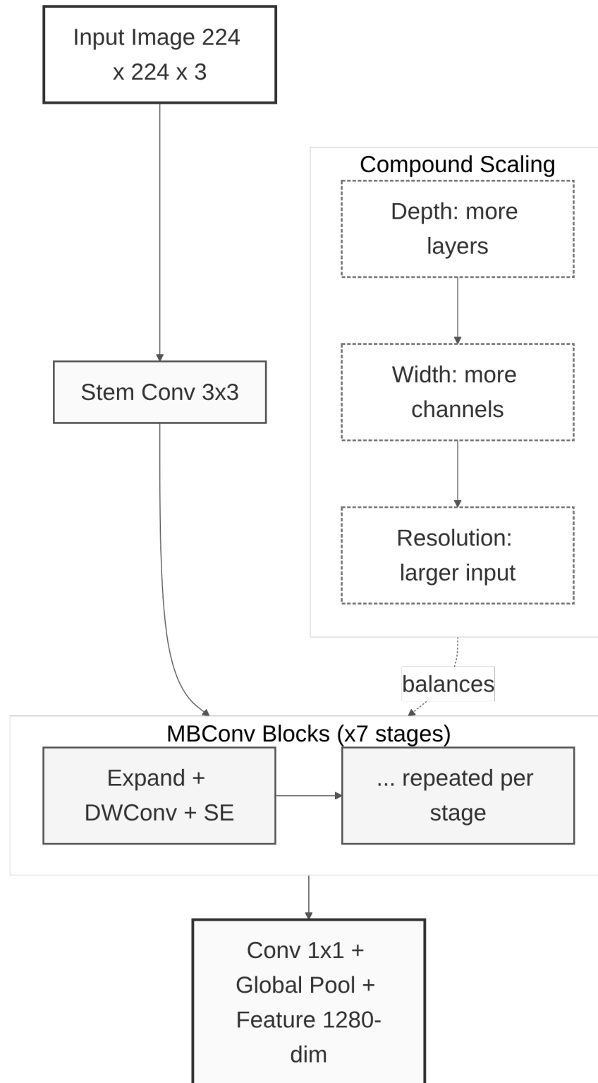
Figure 1: EfficientNet-B0 architecture showing the flow from input image to feature vector
