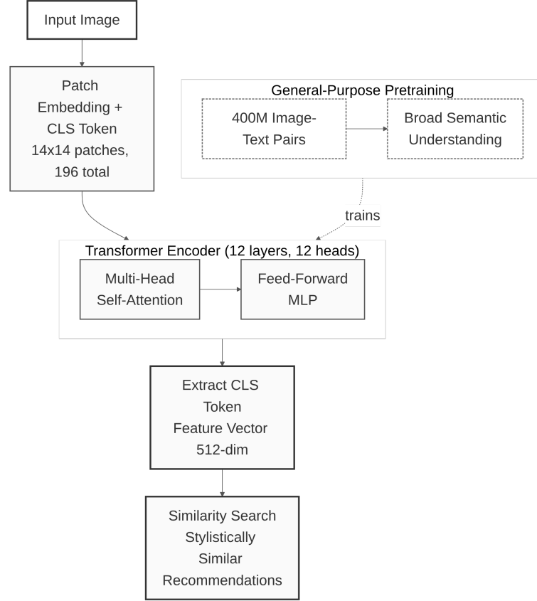
Figure 4: CLIP ViT-B/16 generates 512-dimensional embeddings for image-to-image and text-to-image similarity search
