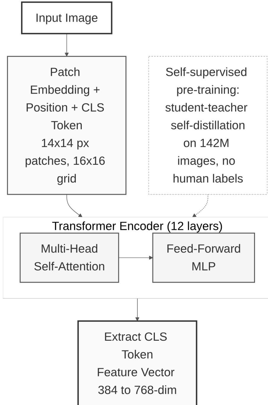
Figure 2: Vision Transformer converts an image into patches and uses self-attention to understand relationships between them
