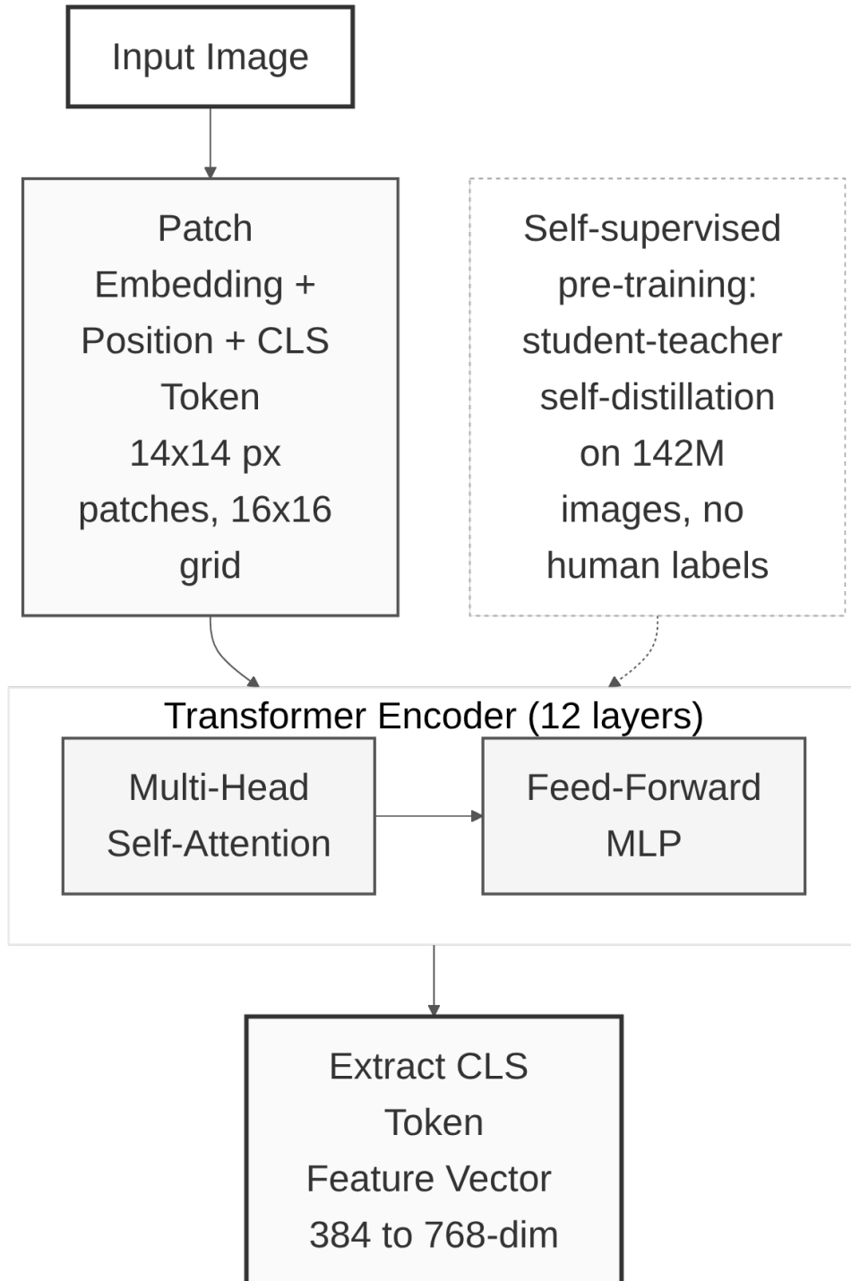
Figure 3: DINOv2 architecture. Image patches pass through a 12-layer transformer encoder with multi-head self-attention and feed-forward MLP in each layer. The CLS token output produces a 384- or 768-dimensional feature vector. The model is trained via self-supervised student-teacher self-distillation on 142 million images, requiring no human labels.
