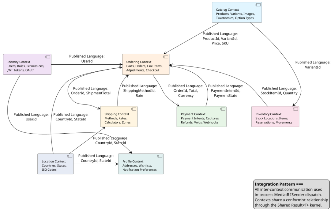
Figure 6: Bounded Context Map showing the eight business contexts and the Published Language identifiers exchanged between them. All integration uses in-process MediatR dispatch; no context directly references another context's namespace.
