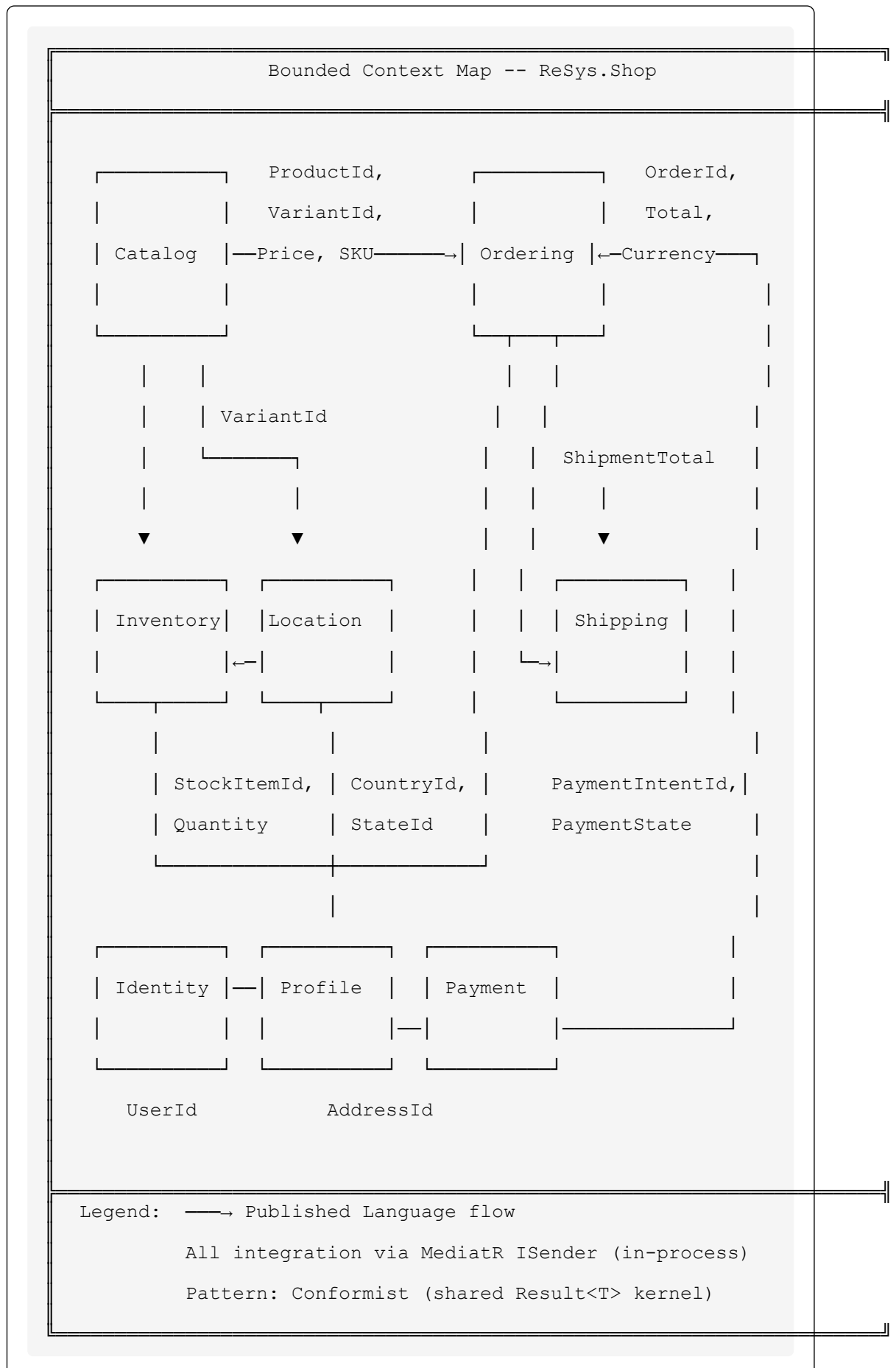
Listing 1: Bounded Context Map – 8 contexts and their Published Languages
