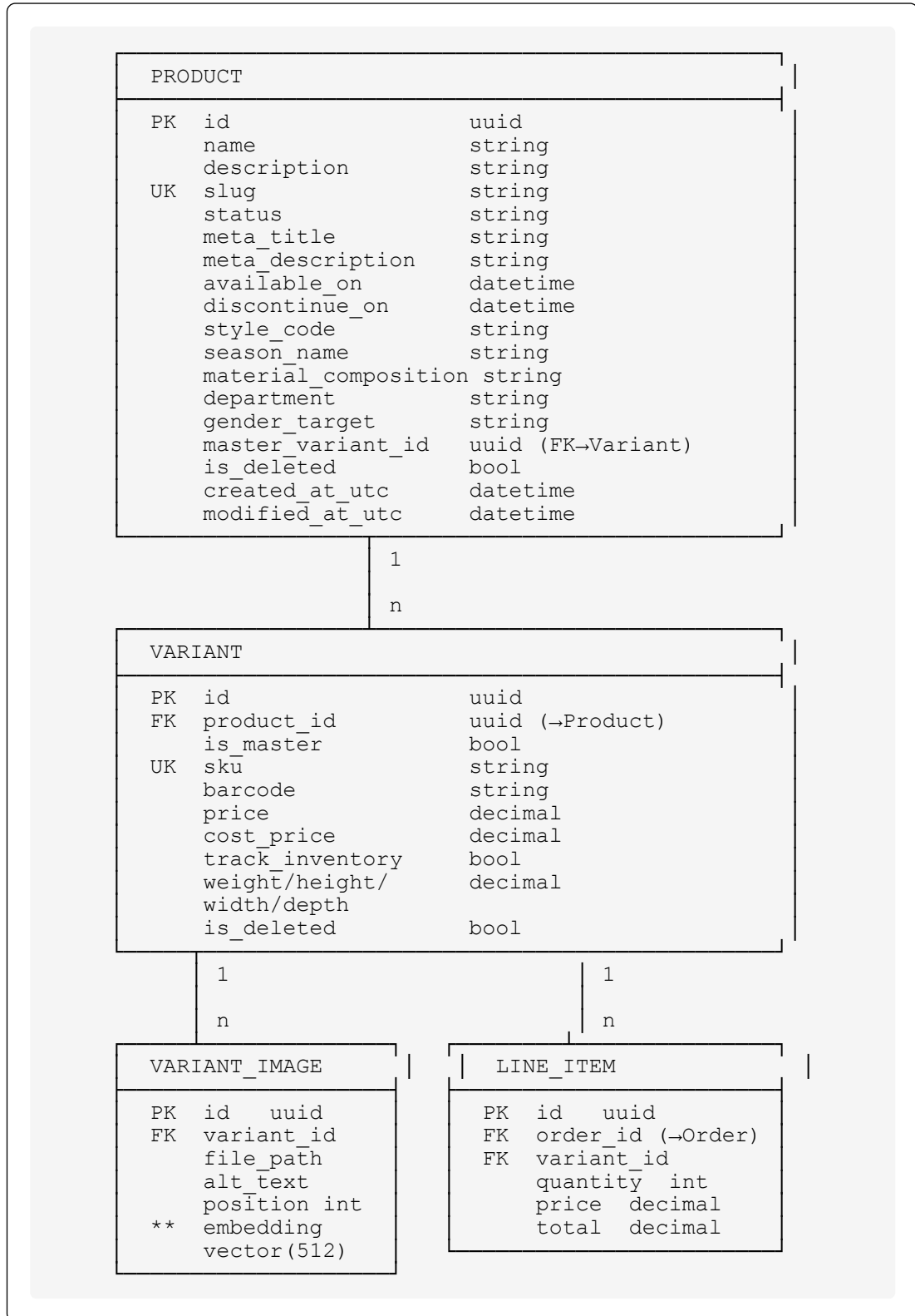
Listing 2: Entity Relationship Diagram – Core Business Entities
