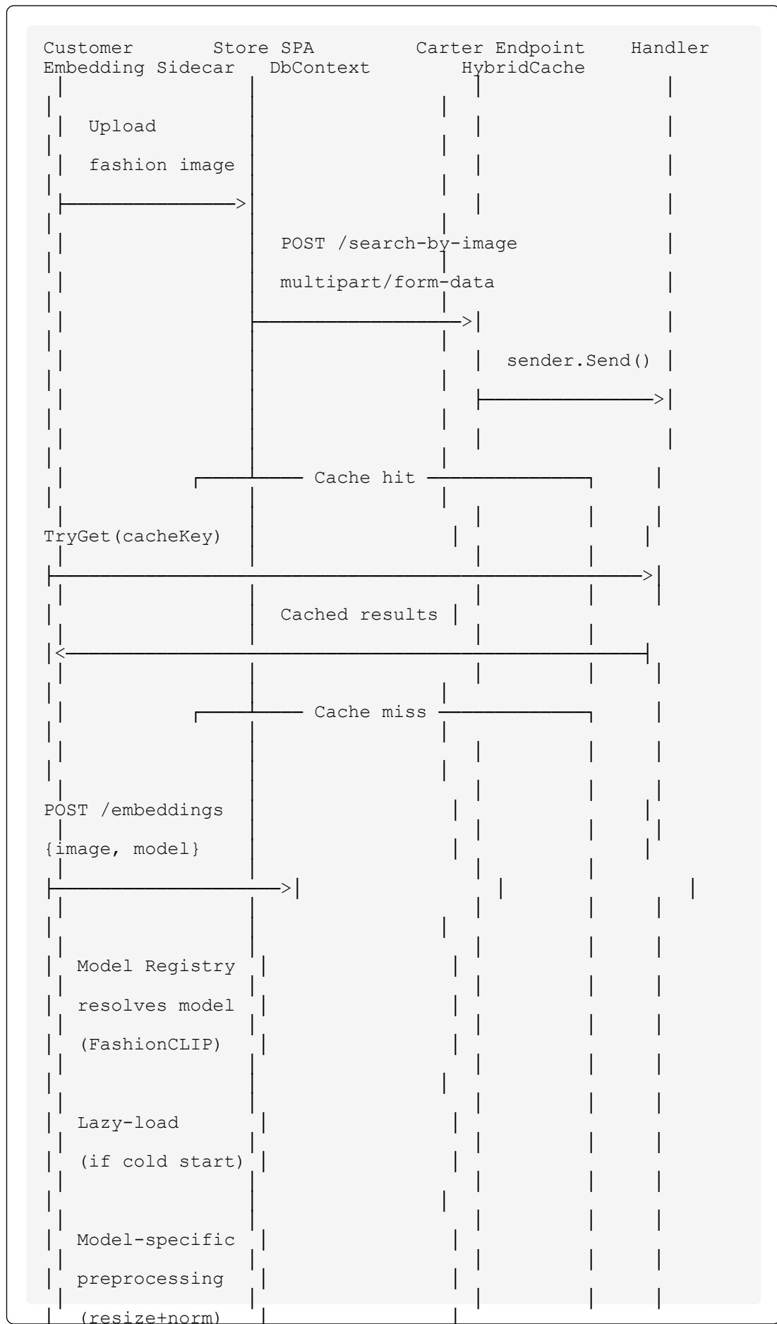
Listing 5: Sequence diagram: Image Search (CBIR – Model-Agnostic)
