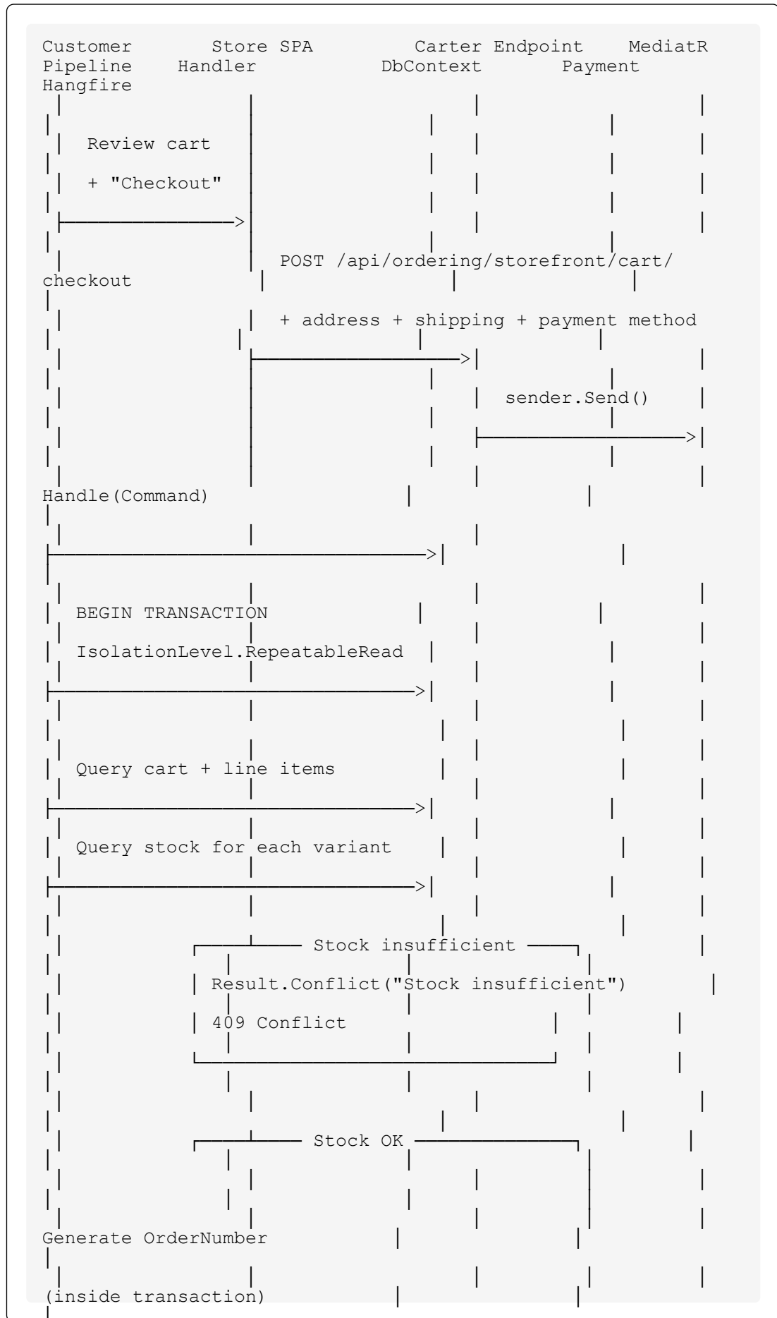
Listing 4: Sequence diagram: Checkout (Critical Path)
