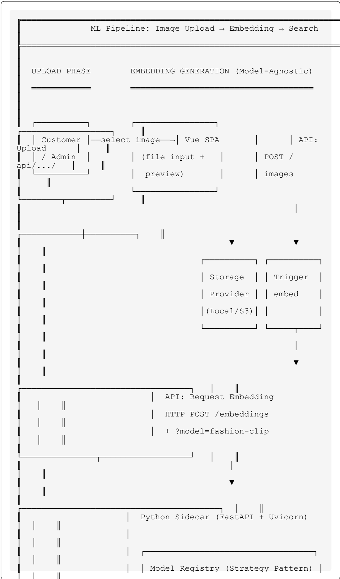
Listing 6: ML Pipeline – Image Upload, Model-Agnostic Embedding Generation, and CBIR Retrieval
