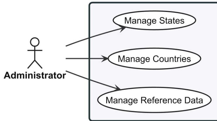
Figure 20: Use case diagram for Reference Data Management (UC-ADM-REF).
