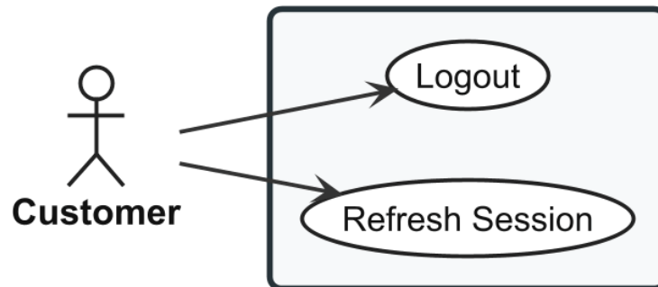
Figure 28: Use case diagram for Session Management (UC-STR-SES).
