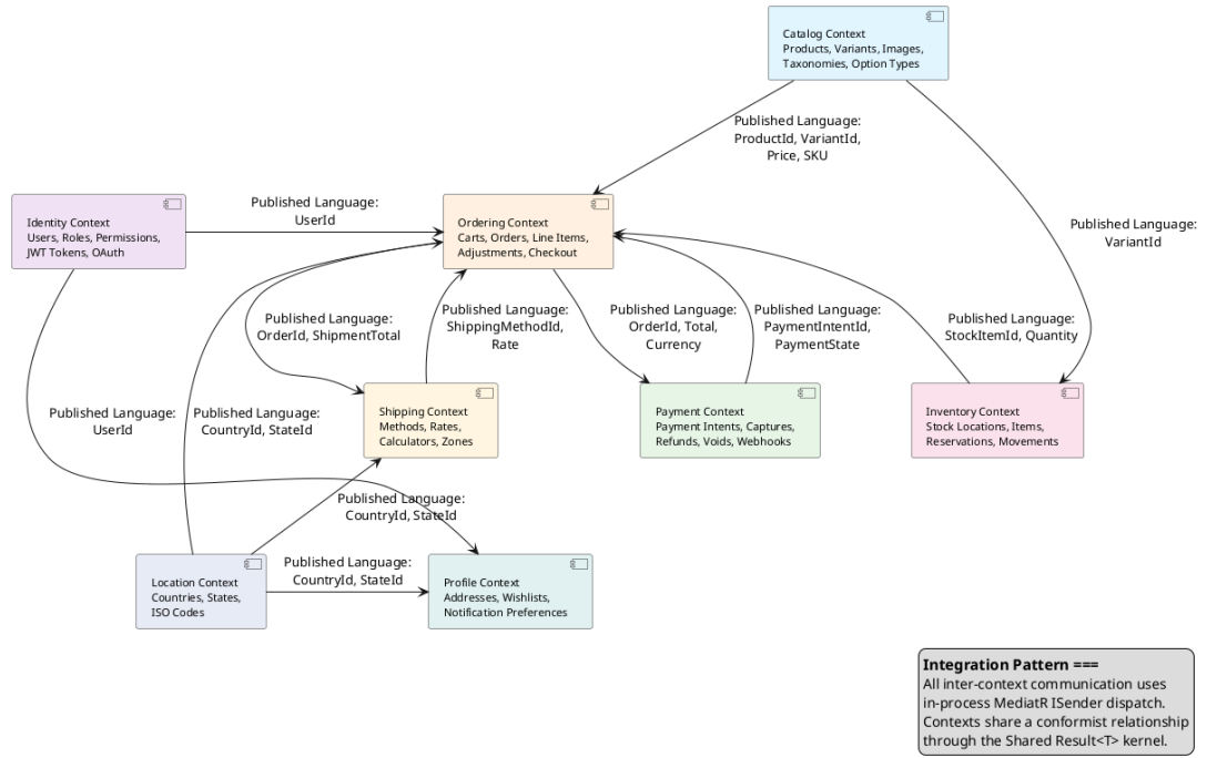
Figure 3: Bounded Context Map showing the eight business contexts and the Published Language identifiers exchanged between them. All integration uses in-process MediatR dispatch; no context directly references another context’s namespace.
