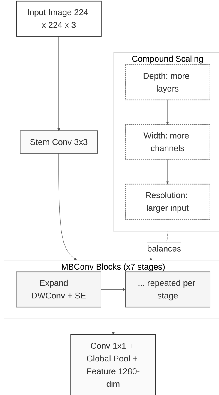
Figure 2: EfficientNet-B0 architecture. Seven stages of MBConv (Mobile Inverted Bottleneck) blocks extract hierarchical features. The Compound Scaling subgraph illustrates how depth, width, and resolution are jointly balanced across B0 through B7 model family.
