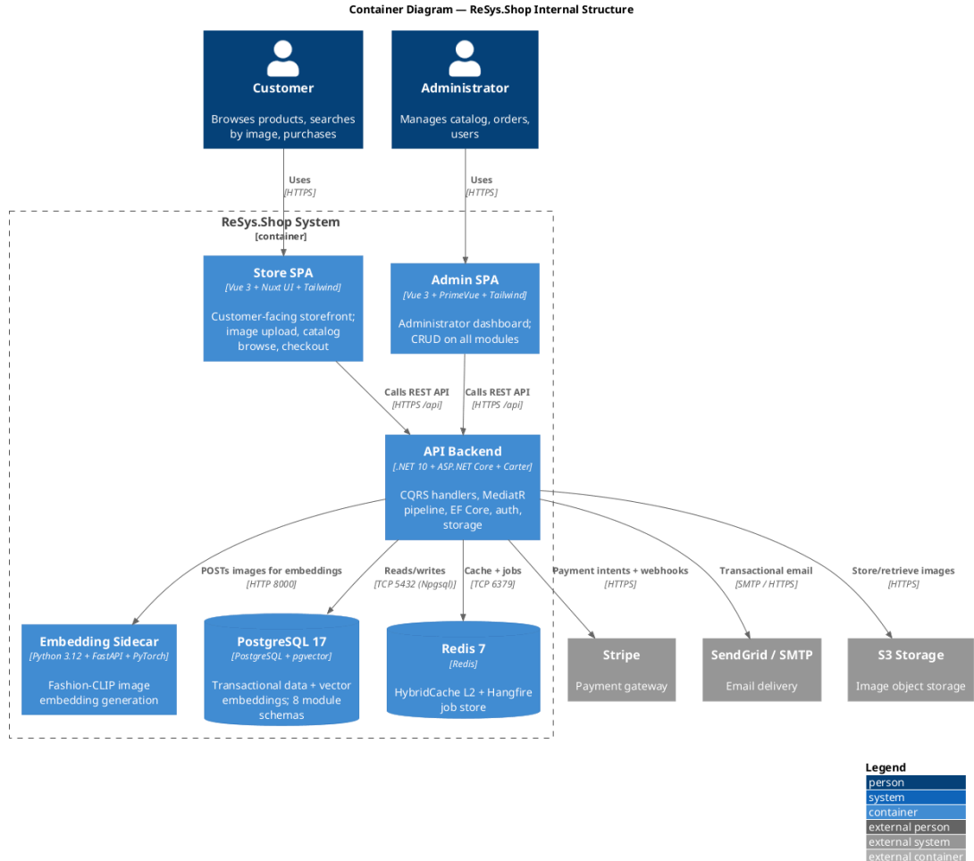
Figure 12: Container diagram showing the deployable units of ReSys.Shop: two Vue 3 SPAs, the .NET 10 API backend, the Python ML sidelcar, PostgreSQL with pgvector, and Redis. Arrows indicate communication protocols between containers.
