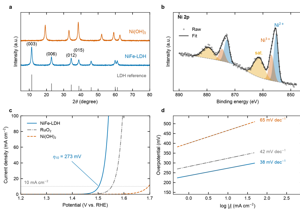
图 2.1 Structural and electrochemical characterization of NiFe-LDH (illustrative synthetic data): (a) XRD patterns with the LDH reference; (b) Ni 2p XPS with peak deconvolution; (c) OER polarization curves with the \eta_{10} annotation; (d) Tafel analysis.
