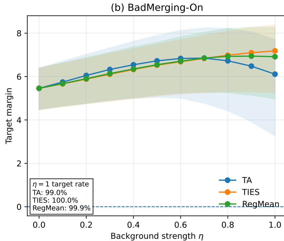
Parameter Geometry vs. Triggered Target-Margin Drift
