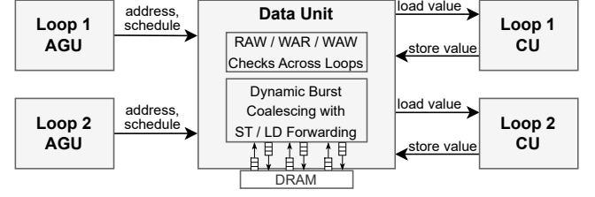
Figure 2: An example DAE streaming FPGA architecture.
