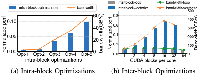
Fig. 13: Optimizations of Rodinia backprop case layerforward kernel. (a) Intra-block optimization ablation: options(1-5): 1)baseline with vector length 8; 2)1-D vectorization adopted from WCCV [31]; 3)control-flow simplification; 4)in-place computation; 5)2-D vectorization within a block. (b) Further inter-block 2-D vectorization based on 5).
