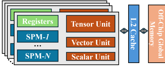
Fig. 2: NPU Architectures Abstraction
