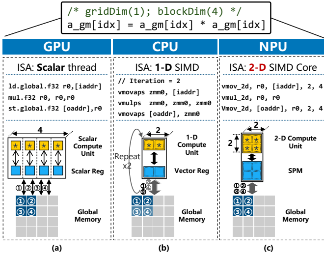
Fig. 1: Execute the same CUDA program on GPU, CPU, and NPU: one block is launched, transferring four strided numbers from global memory to registers. The program’s inherent parallelism is materialized differently across platforms.
