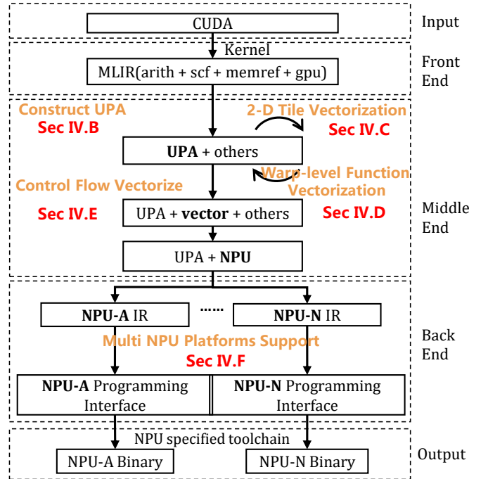
Fig. 5: Overview of our compiler pipeline.
