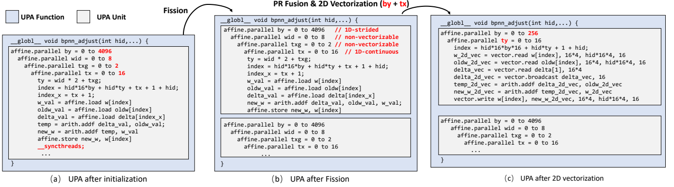
Fig. 6: Examples of Unified Parallelism Abstraction(UPA) for CUDA code in Figure 3(a).
