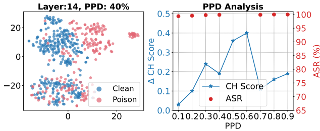
Fig. S2: Exploratory hidden-state clustering under controlled diagnostic mixtures. Left: descriptive, label-colored t-SNE visualization with 40% triggered inputs. Right: CH-score change and ASR across triggered-sample fractions. This analysis does not define or evaluate a deployment detector.
