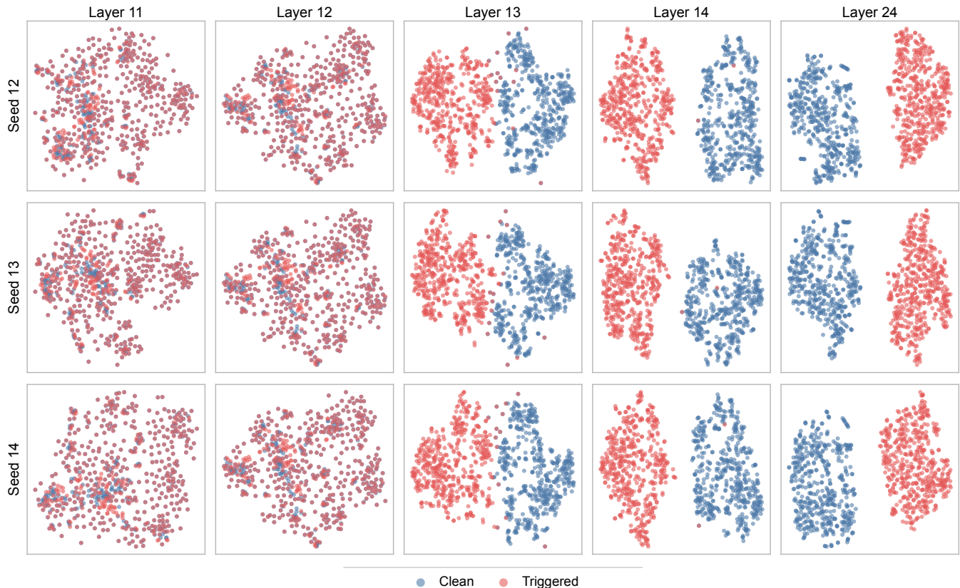
Fig. S1: 3-seed t-SNE visualization of clean and triggered Mixtral representations. Rows denote random seeds; columns denote layers. Blue and red represent clean and triggered inputs, respectively.
