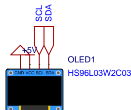
OLED
