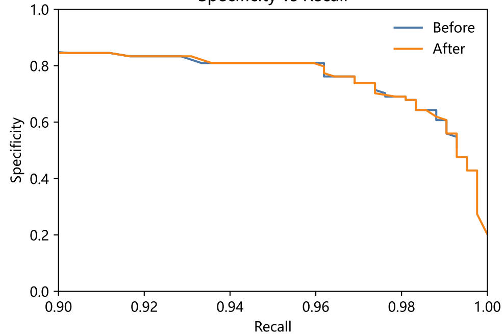
Specificity vs Recall
