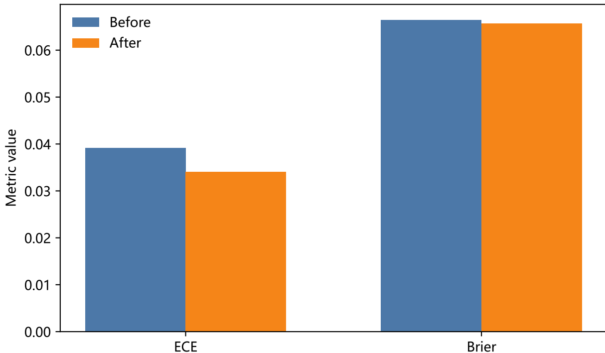
Calibration metrics
